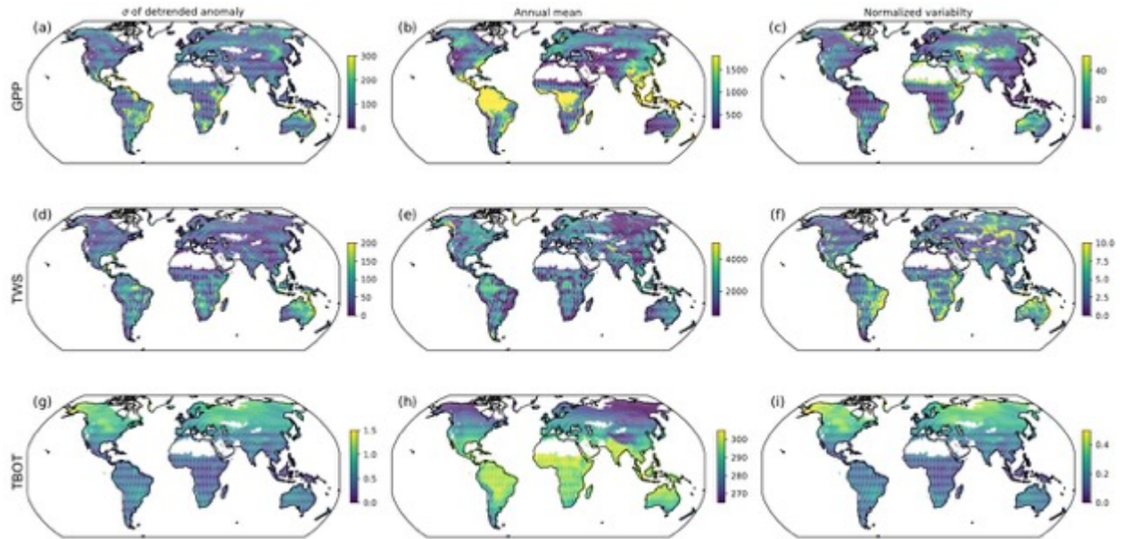
Figure S5. Characterization of GPP (top row), terrestrial water storage (TWS, middle row), and air temperature (TBOT, bottom row) simulated by CESM2-ESM. The first column (a, d, g) shows the standard deviation of detrended annual anomalies (units: \text{gC m}^{-2} \text{y}^{-1} , \text{kg H}_2\text{O m}^{-2} , and K, respectively) The second column (b, e, h) shows the annual mean simulated between 1960-2014 (units: \text{gC m}^{-2} \text{y}^{-1} , \text{kg H}_2\text{O m}^{-2} , and K, respectively). The third column (c, f, i) shows coefficient of variation (the units %, calculated and the quotient of first and second columns \times 100 ).
