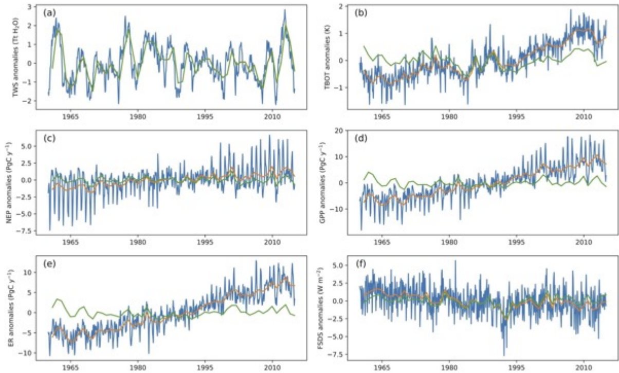
Figure S1. Global monthly anomalies, annual anomalies, and detrended annual anomalies (blue, yellow and green lines respectively). Panels show variability in globally summed: (a) terrestrial water storage (TWS); (b) Air temperature (TBOT); (c) Net ecosystem production (NEP); (d) Gross primary productivity (GPP), (e) Ecosystem respiration (ER); and (f) globally averaged incoming solar radiation (FSDS) that was simulated over vegetated terrestrial grid cells by from CESM2-ESM simulations over the end of the historical period (1960-2014).
