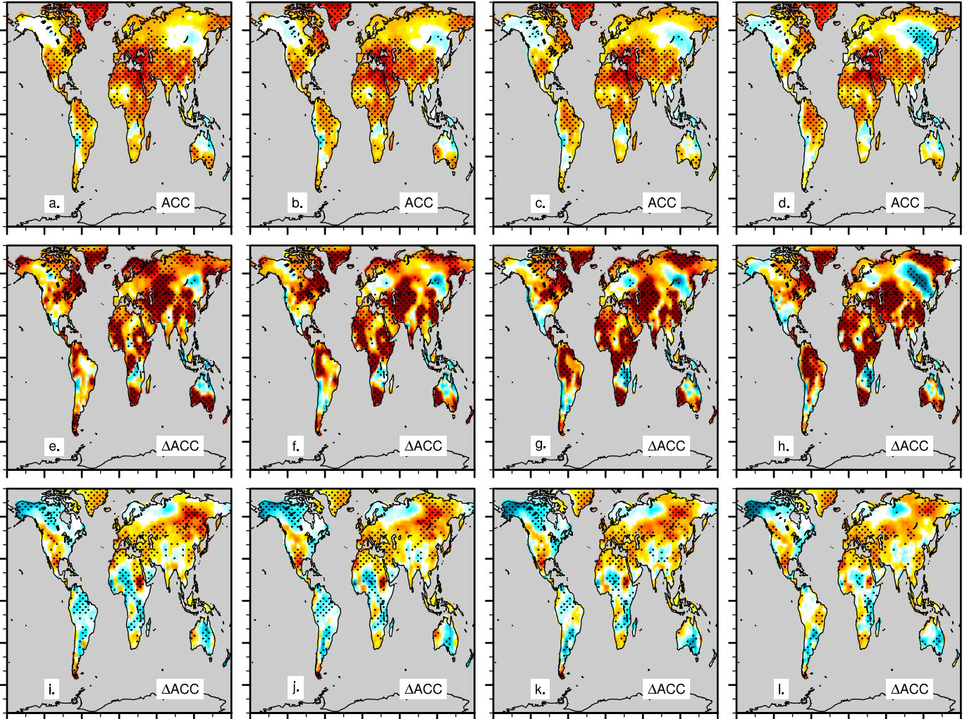
ACC, Surface Air Temperature, OBS=CRU-TS4.0, Season=ANNUAL, (LY 3-7: 1959.5-2013.5), detrended LY 3-7 LY 4-8 LY 5-9 LY 6-10
