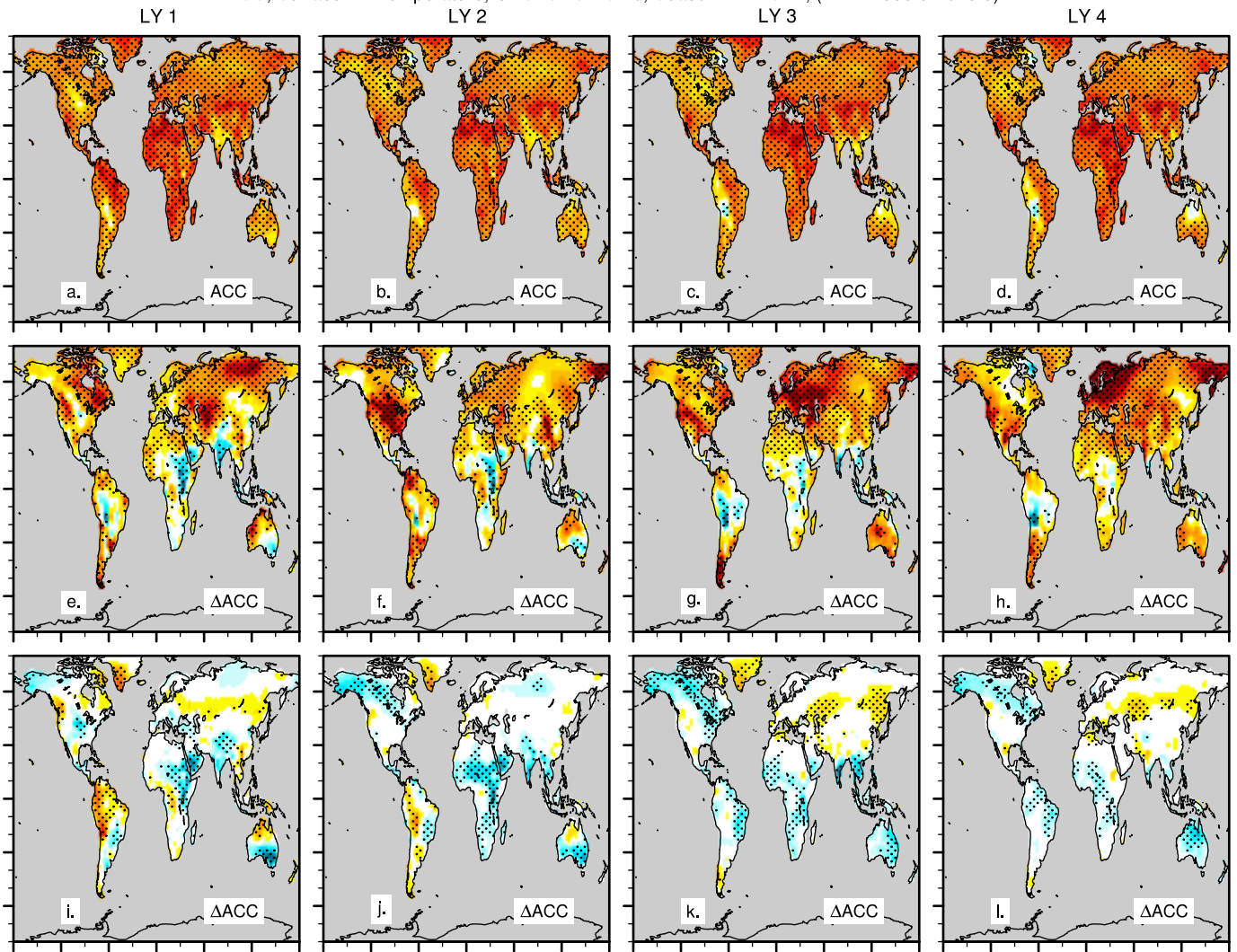
ACC, Surface Air Temperature, OBS=CRU-TS4.0, Season=ANNUAL, (LY 1: 1955.5-2015.5)
