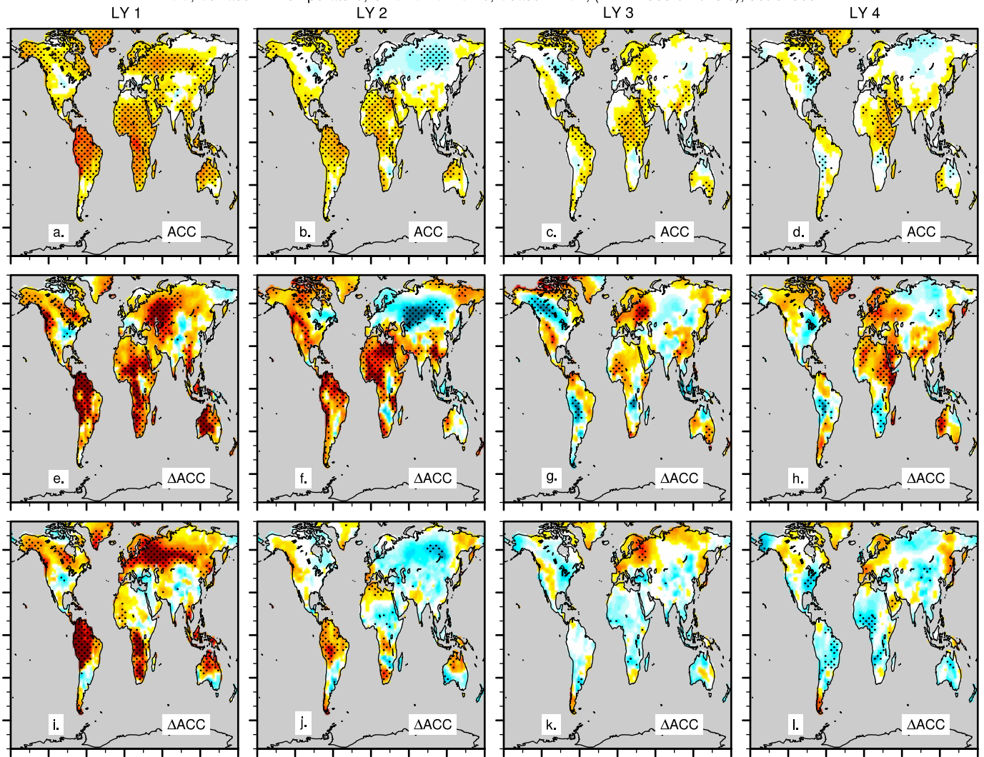
ACC, Surface Air Temperature, OBS=CRU-TS4.0, Season=DJF, (LY 1: 1955.0-2015.0), detrended
