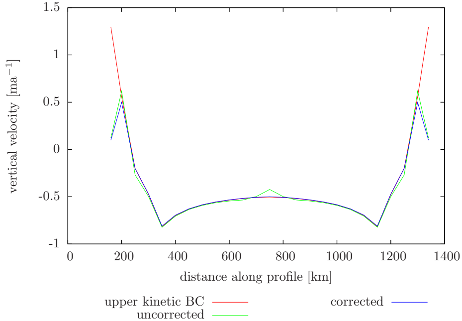
Figure 3.6: Vertical ice surface velocities of the EISMINT-1 moving margin experiment.
