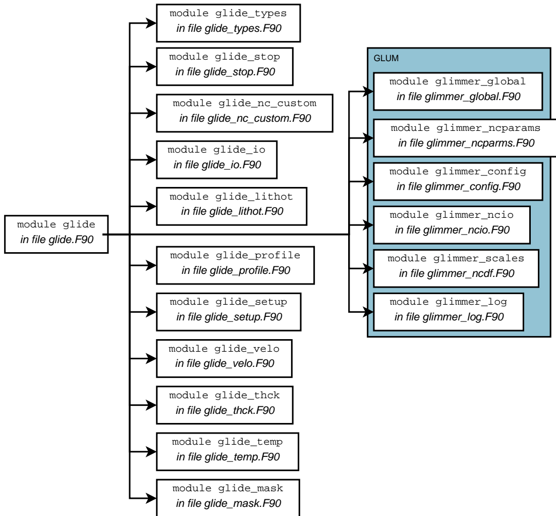
Figure 4.3: Direct module dependency diagram for module glide only, illustrating the complexity of module dependencies.
