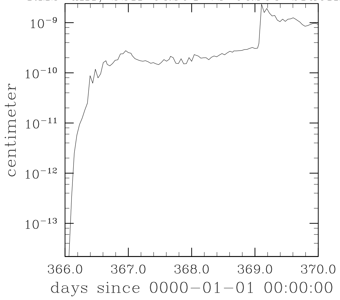
Sea Surface Height RMS diff, SSH Case4 vs Case5 bluefire
