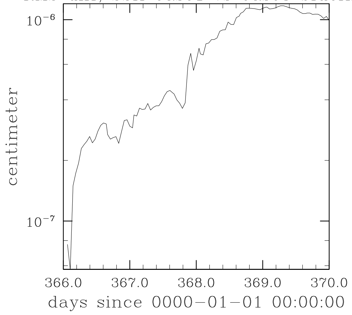
Sea Surface Height RMS diff, SSH Case1 vs Case3 bluefire
