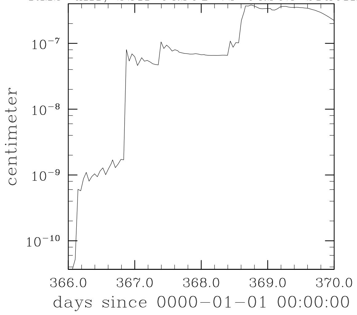
Sea Surface Height RMS diff, SSH Case1 vs Case2 bluefire
