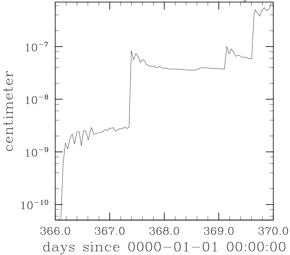
Sea Surface Height RMS diff, SSH Case1 bluefire vs yellowstone
