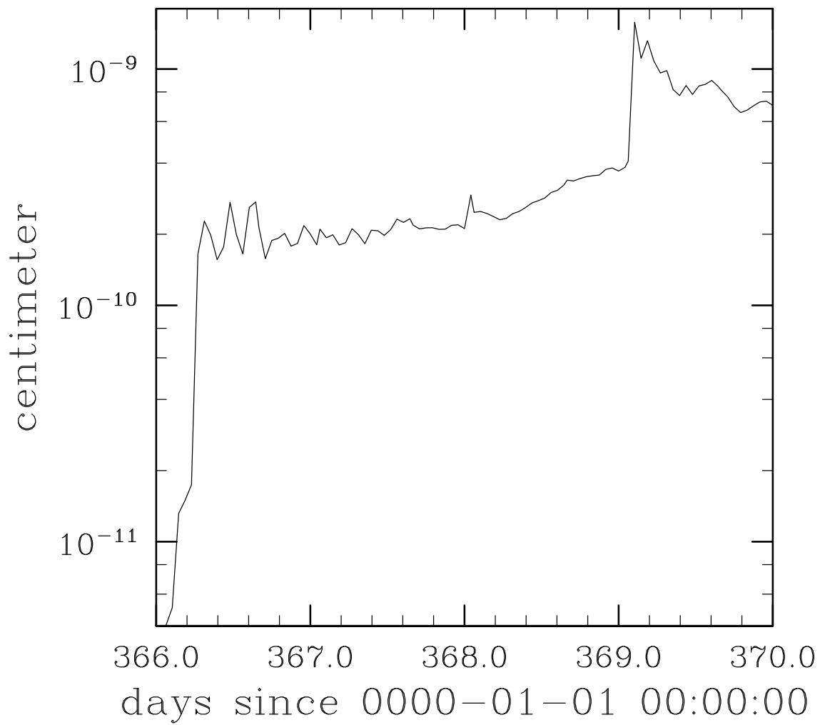
RMS Diff SSH Case4 bluefire vs jaguar
